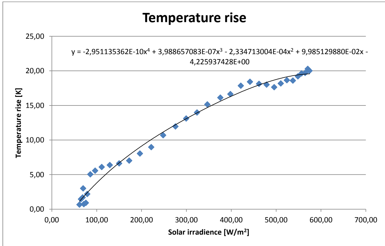
Figure 4 - Temperature rise
