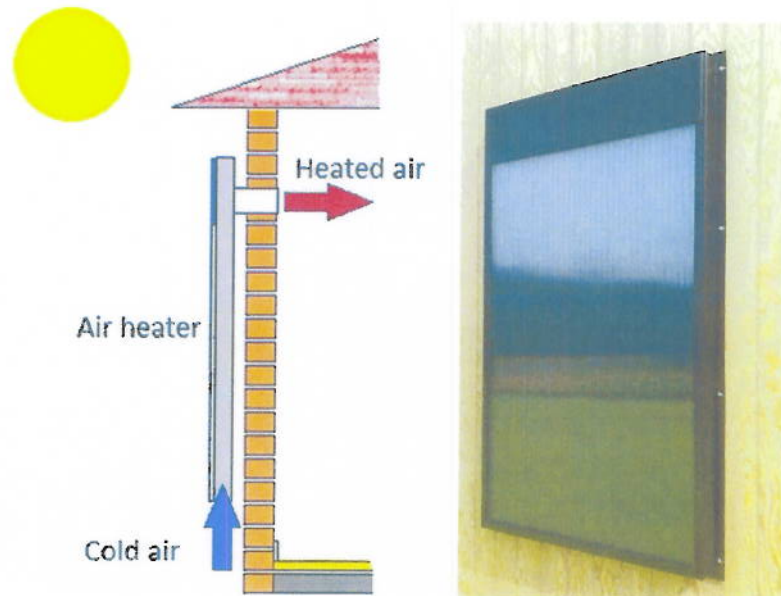
Figure 1: Drawing depicting the function of a solar air heater (left) and the DSB2 solar air heater (right).
